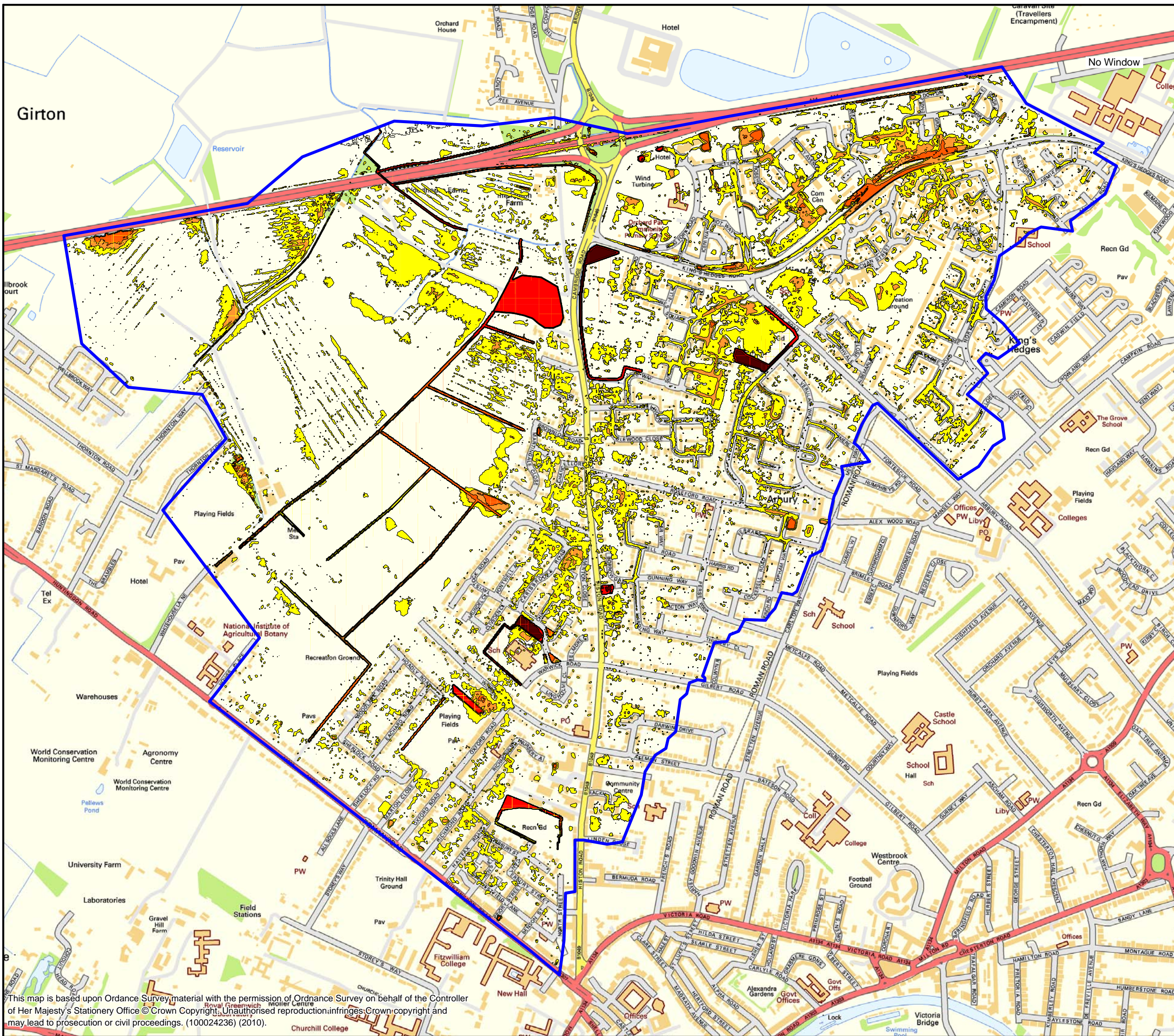
FIGURE F22 0.5% AEP "ENGINEERING OPTION C6" PLUVIAL MODELLING MAXIMUM DEPTH KING'S HEDGES AND ARBURY
